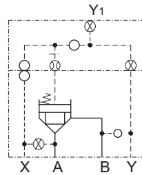
Subplate mounting
