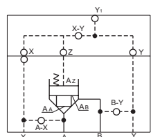
Subplate mounting
