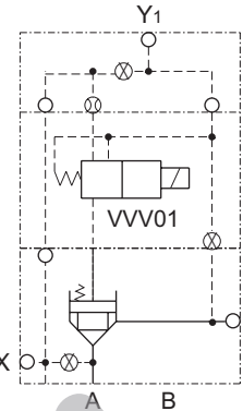
Threaded body
